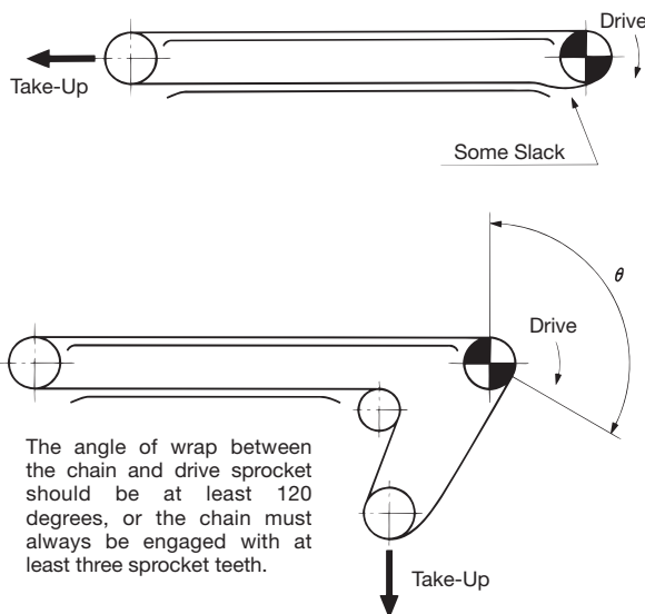
Figure 27: Adjusting Chain Slack
